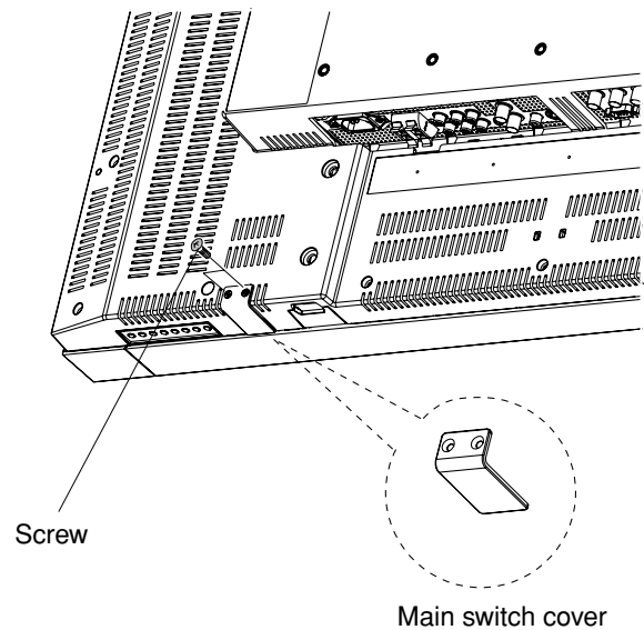
Main switch cover installation example (LDT371V)
